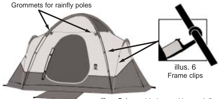
illus. 5 Assembled tent without rainfly. Note the frame clips located on edge of tent.
